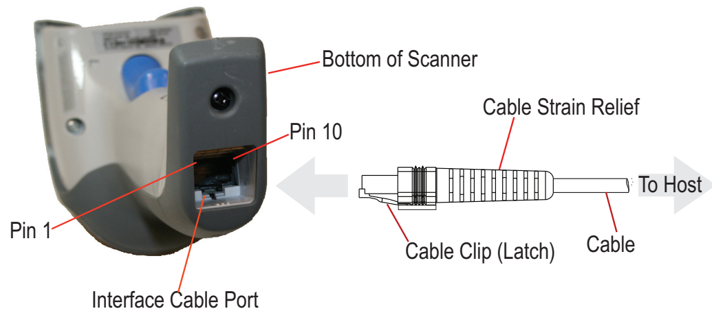
Figure 1. Standard Cable Pinouts: Handheld
