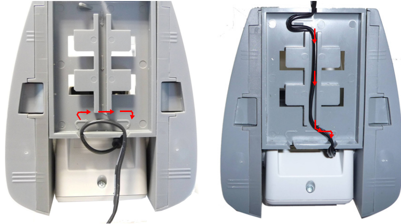
Figure 8. Options for routing the DC cord
