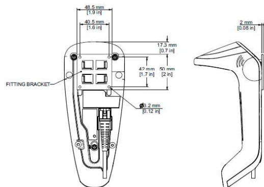
Figure 2 - Vertical Position
