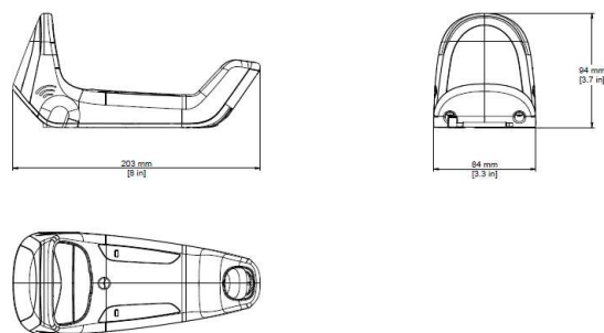
Figure 1 - Horizontal Position
