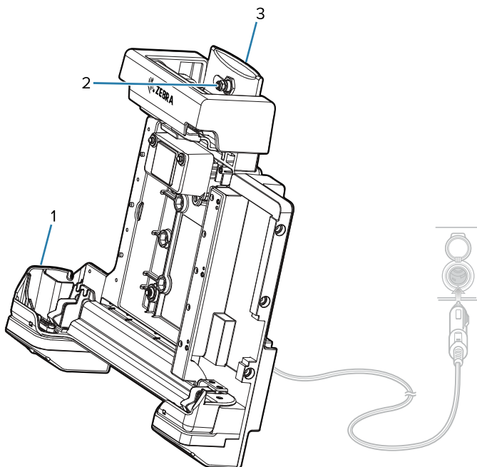
Figure 9 Vehicle Dock Setup
