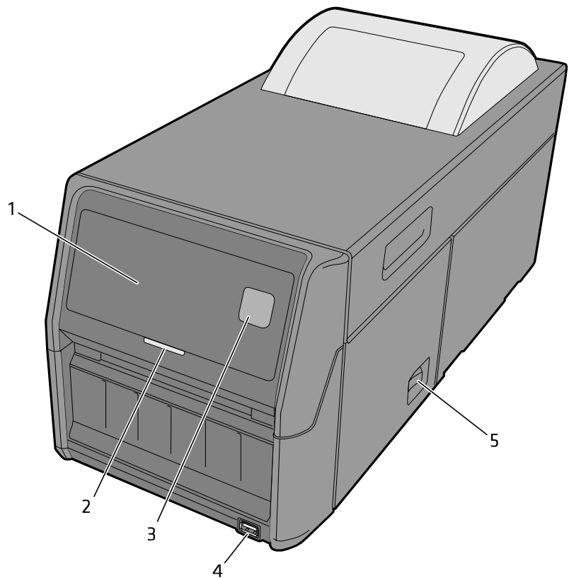
PD43 and PD43c Front Panel Features and Descriptions (Icon Model)
