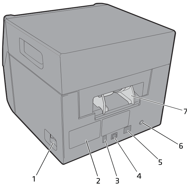
PD43c Rear Panel
