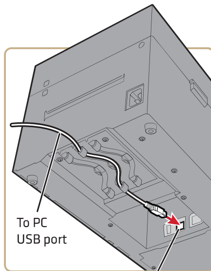
USB device port
