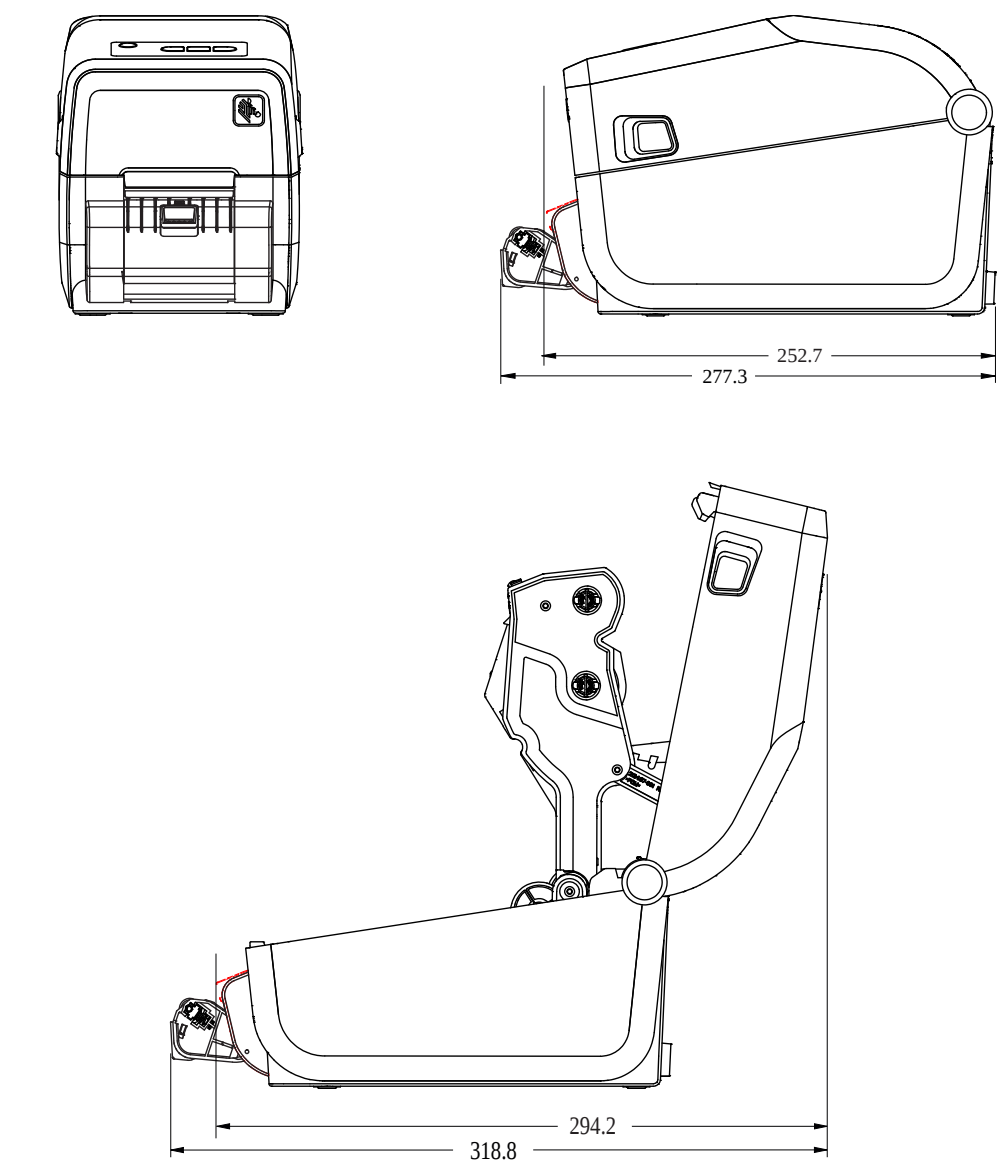
Figure 21 ZD411T Printer with Label Dispense Option (dimensions in millimeters)
