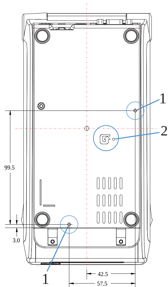
Figure 23 ZD411D Standard Mounting (dimensions in millimeters)
