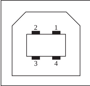
Figure 16 USB -B
