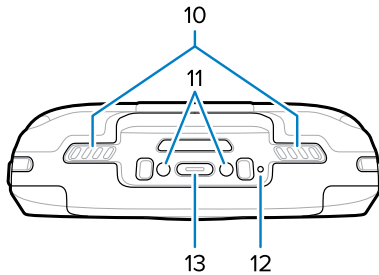
Figure 3 Bottom Views
