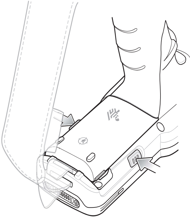
Figure 18 Release Battery
