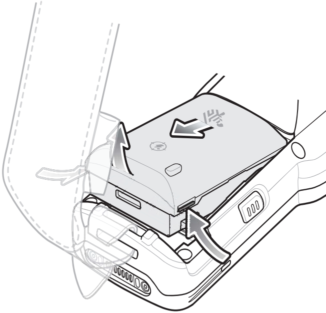
Figure 19 Remove Battery
