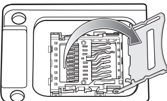
Figure 10 Lift microSD Card Holder
