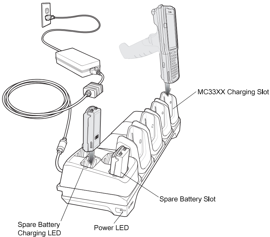
Figure 29 5-Slot ShareCradle with 4-Slot Battery Charger
