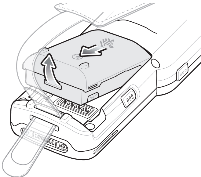
Figure 23 Remove Battery
