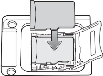
Figure 11 Install microSD Card
