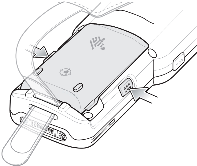
Figure 22 Release Battery
