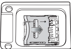
Figure 9 Unlock microSD Card Holder
