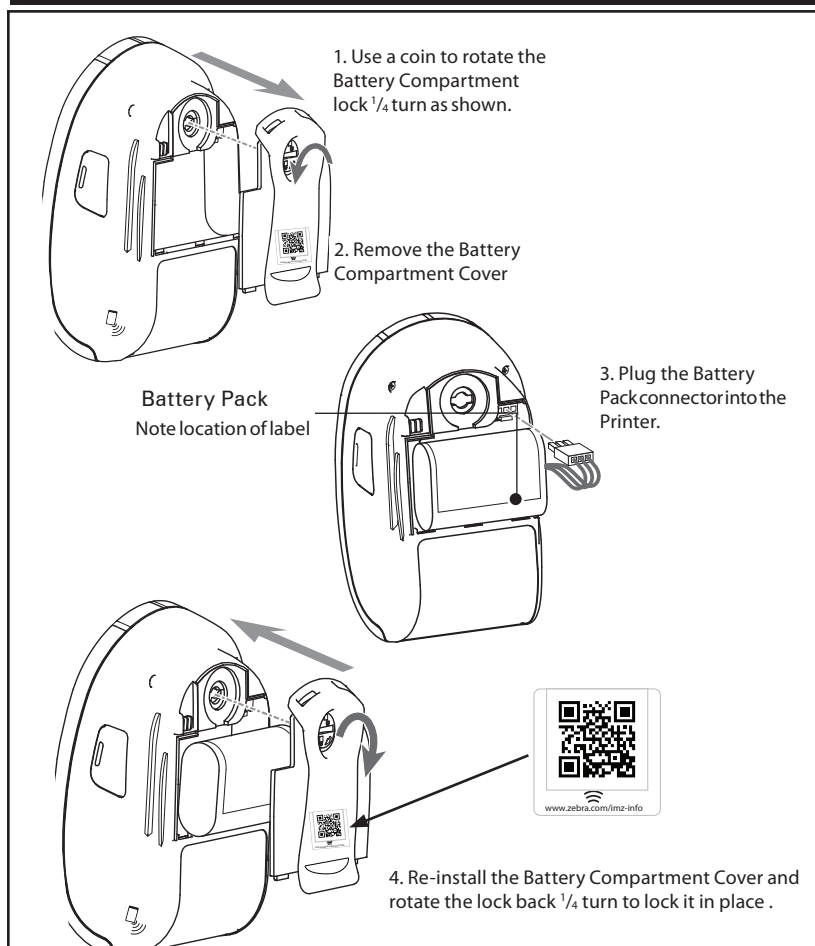
Figure 2.1: Installing the Battery
