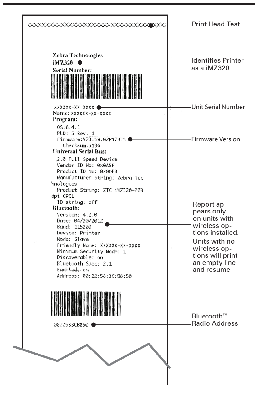
Figure 18: Configuration Label Example (iMZ320 illustrated)
