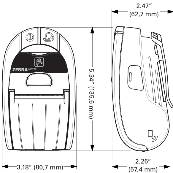
Figure 20 iMZ220 Overall Dimensions
