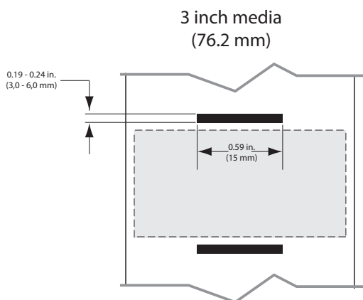
Figure 7: Media Black Bar Dimensions
