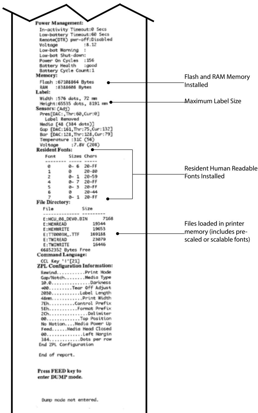
Figure 21c: ZQ500 Series Configuration Label (cont.)
