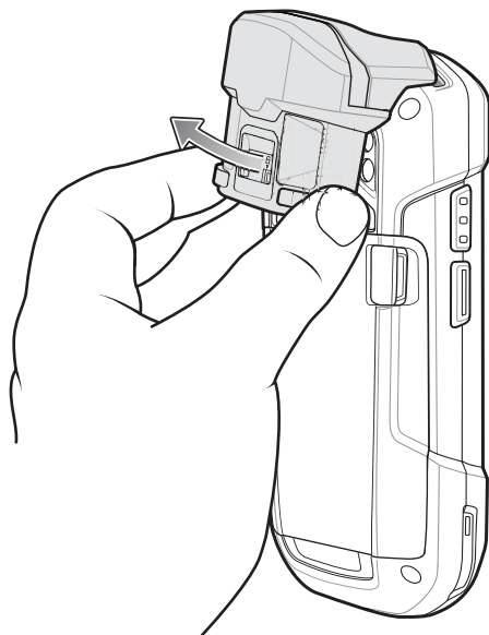
Figure 116: Remove MSR
