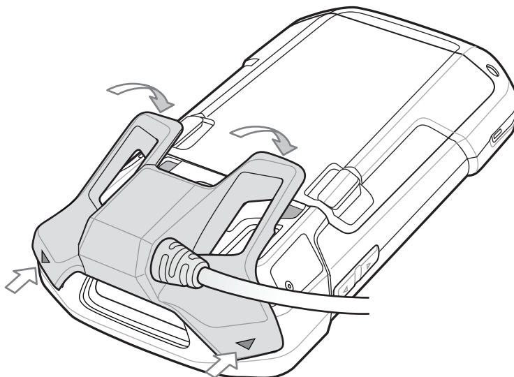
Figure 124: Audio Adapter Installation
