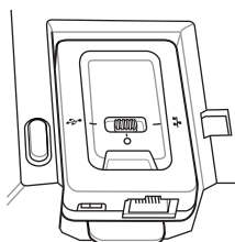
Figure 104: 2-Slot USB/Ethernet Cradle Module Switch
