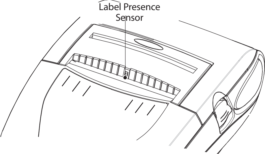
Figure 17.2- Cleaning the P4T Series Peeler Assembly
