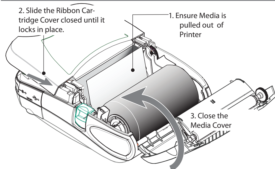
Figure 9.3-Close the Printer Covers
