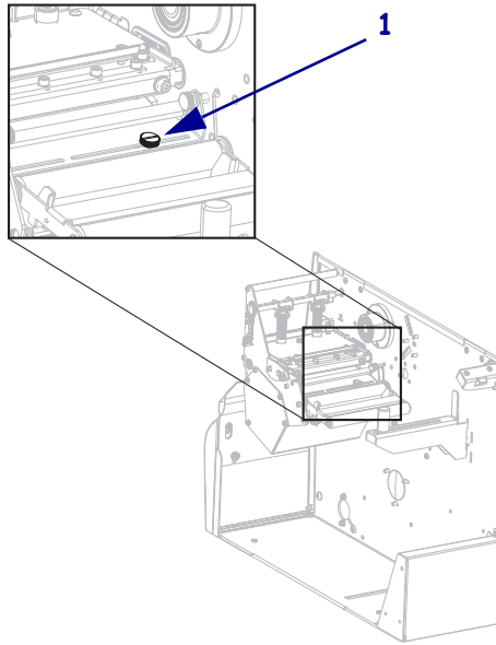
Figure 10 • Upper Media Sensor
