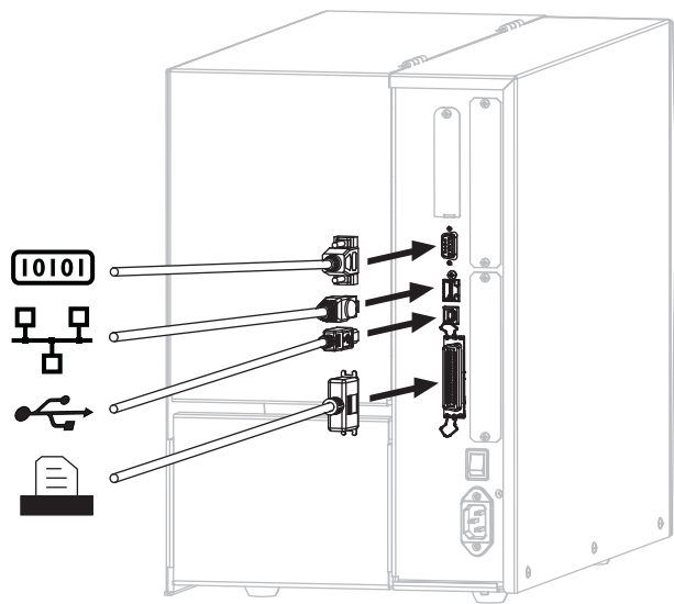
Figure 4 • Communication Interfaces
