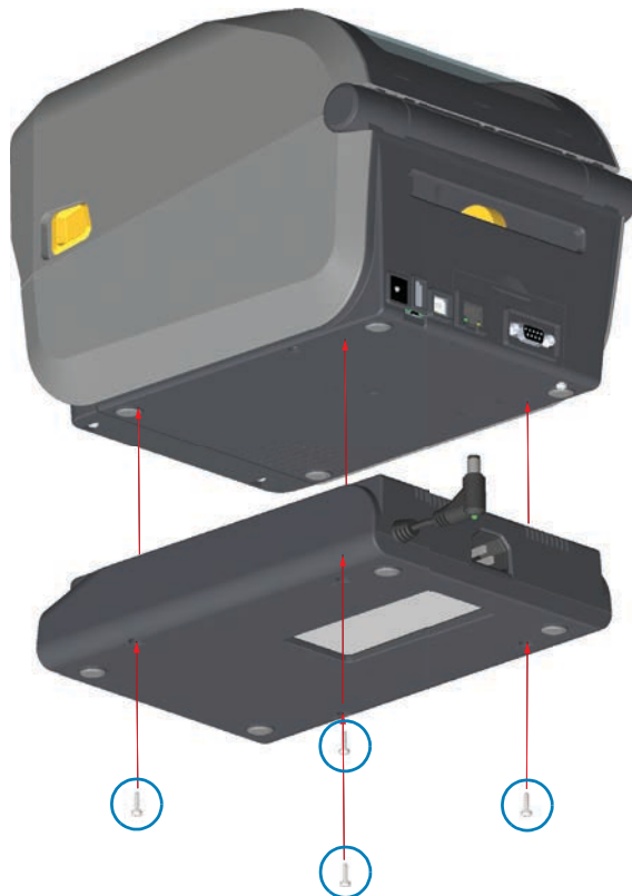
Thermotransferdrucker
