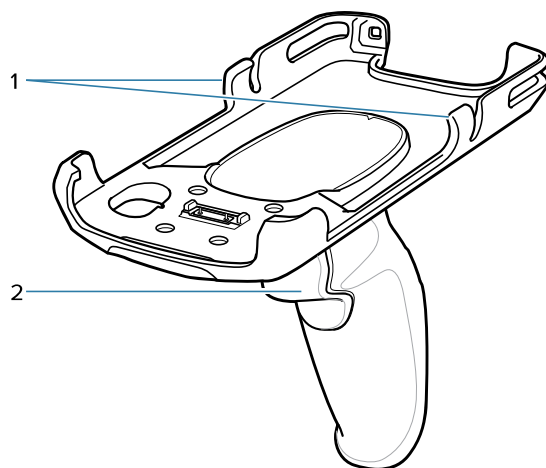
Figure 39 Trigger Handle
