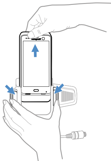
CT45-VD-CNV-SPK
