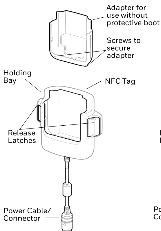
CT40-VD-CNV/CT45-VD-CNV
