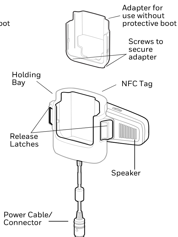
CT45-VD-CNV-SPK
