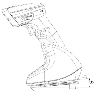
Figure 2 - Tilting Platform Position
