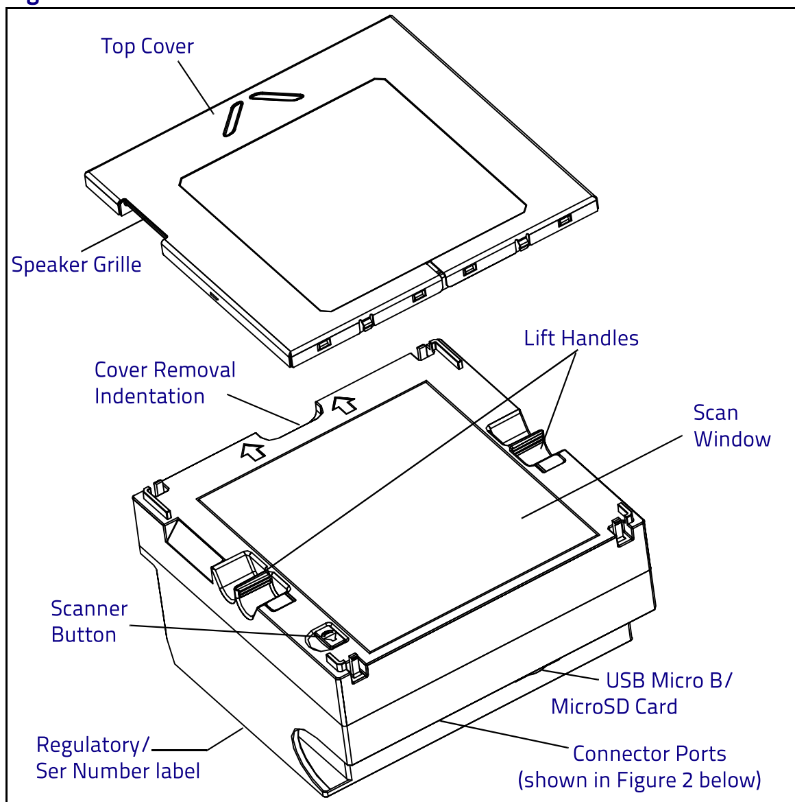
Figure 1. Scanner Features - Front View
