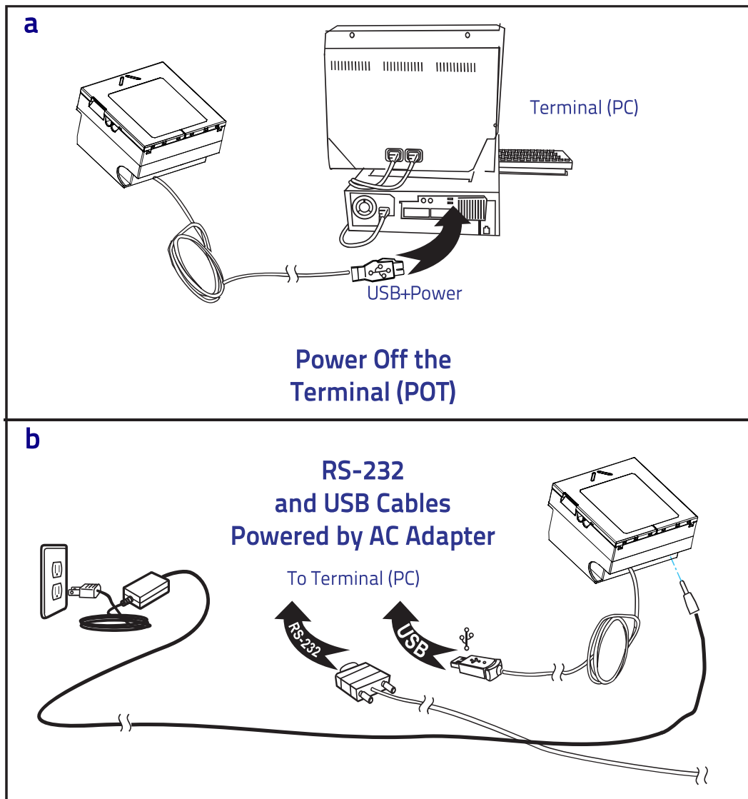
Figure 3. Scanner Cabling
