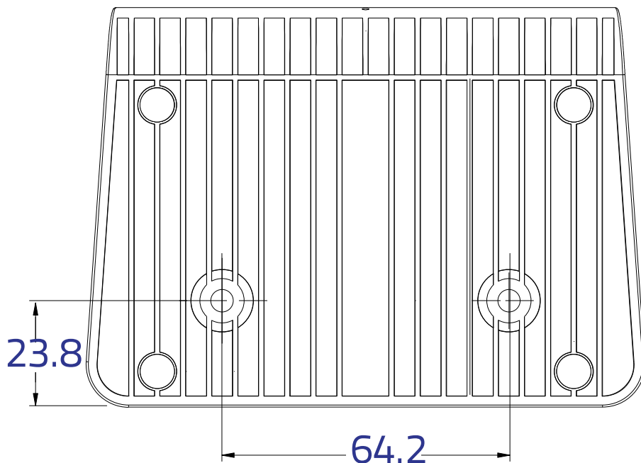
Figure 11. Tilting Riser Dimensions
