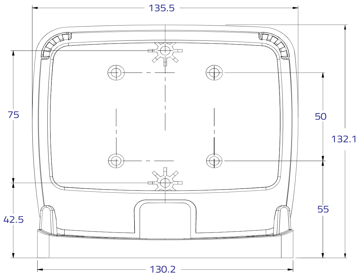
Figure 7. Wall (Vertical) Dimensions
