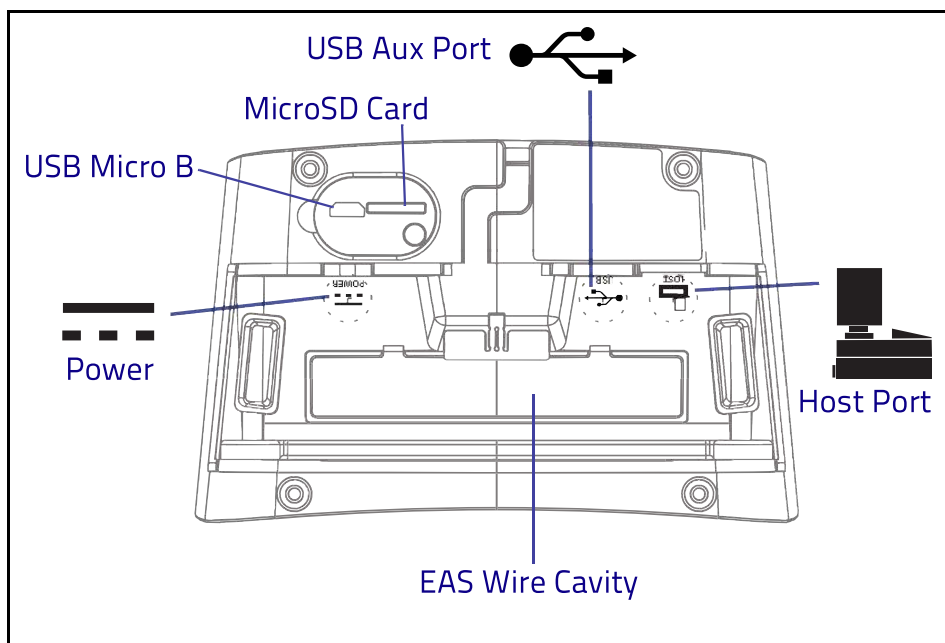
Figure 3. Scanner Features - Bottom View
