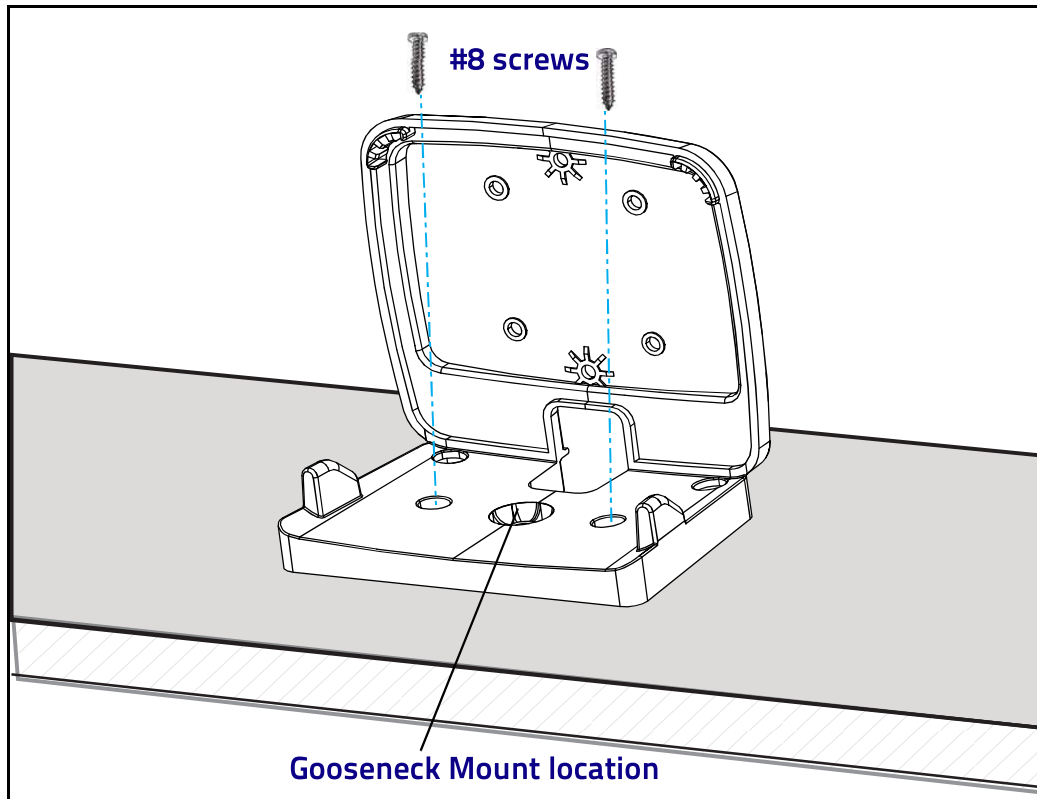
Figure 4. Desk Mount
