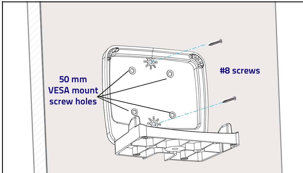
Figure 6. Wall mount
