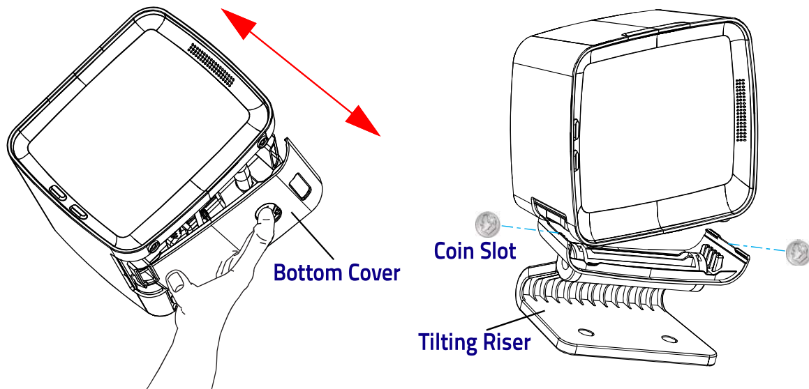
Figure 9. Attaching the Tilting Riser
