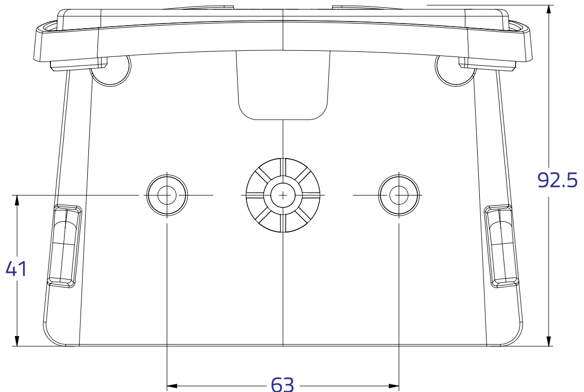
Figure 5. Desk Mounting Dimensions
