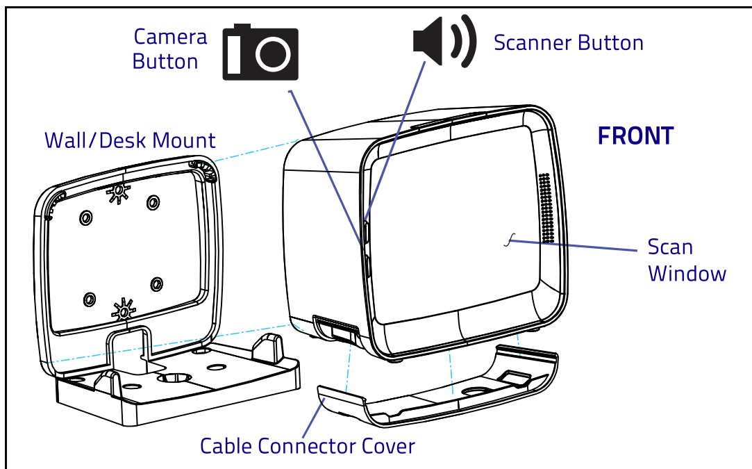
Figure 1. Scanner Features - Front View
