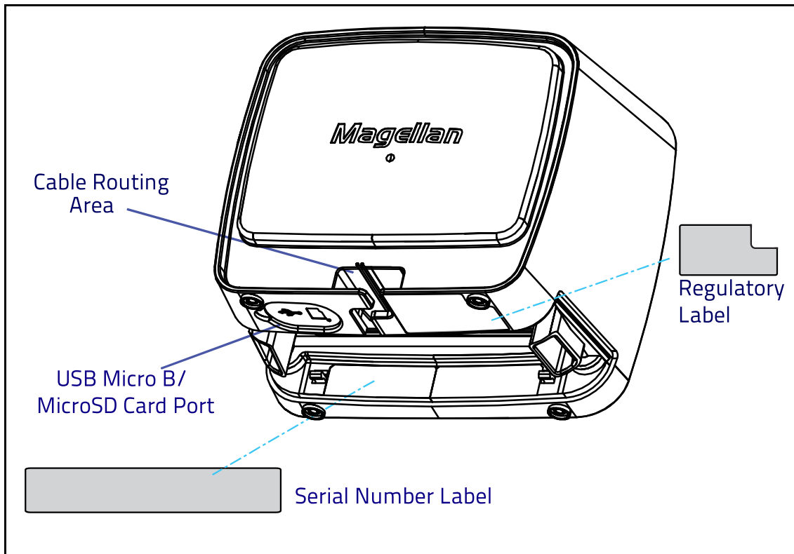
Figure 3. Scanner Features - Bottom View
