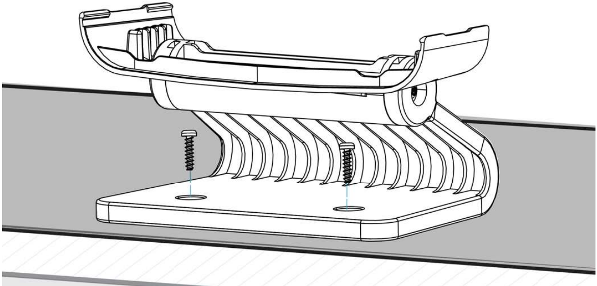
Figure 10. Mounting the Tilting Riser
