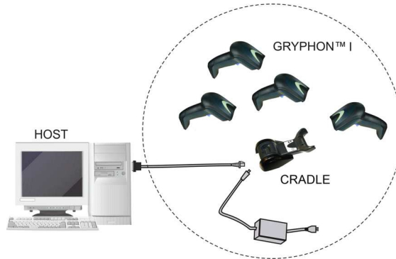
Figure 8. Multiple Reader Layout
